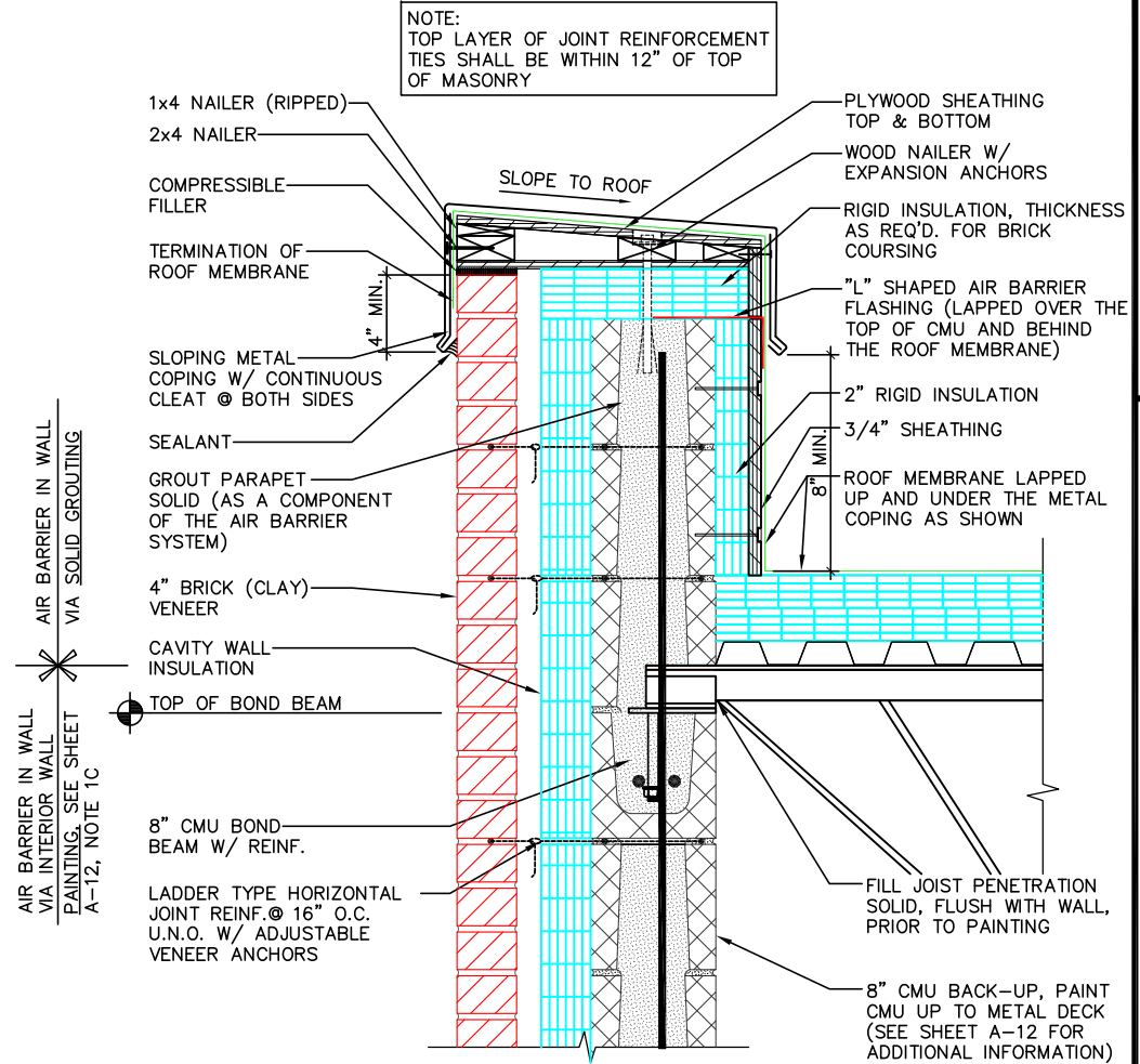
SECTION VIEW
